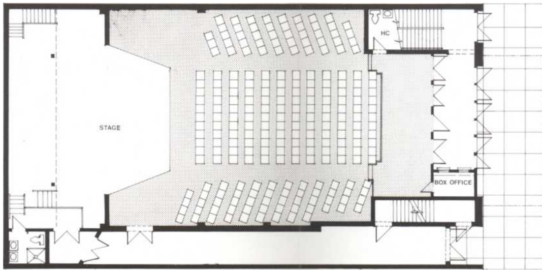
The Lucille Lortel Theatre 121 Christopher Street, NYC Ground Floor Plan
